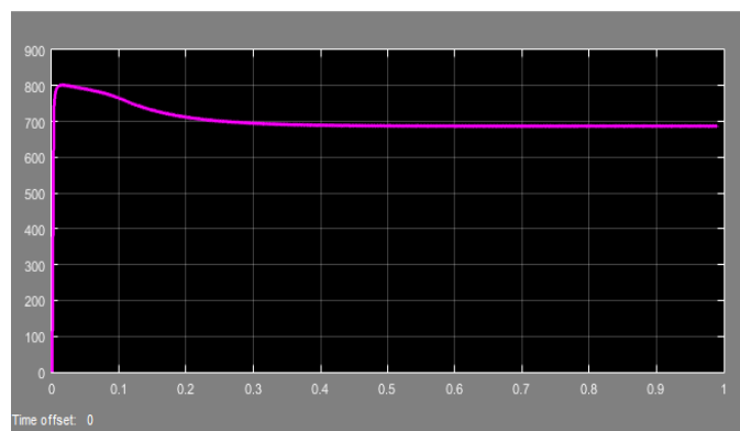
Fig.8. output voltage at input voltage= 40V(Two stage).
