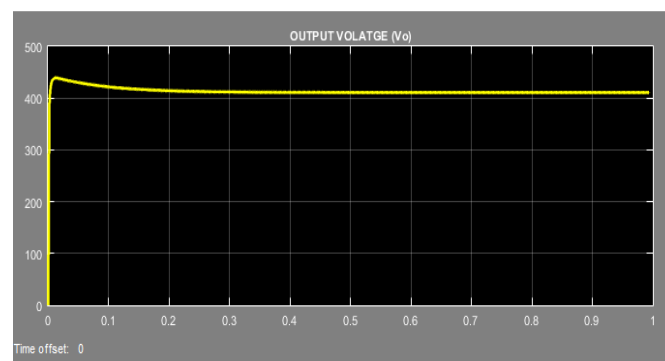
Fig.5. output voltage at input voltage=40V (single stage)
