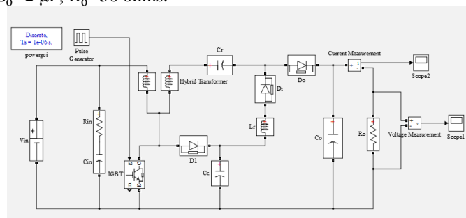
Fig.3. Simulation diagram of proposed high boost ratio hybrid transformer dc-dc converter (single stage)
