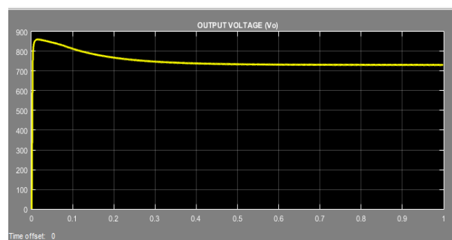
Fig.6. output voltage at input voltage= 40V (Two stage).
